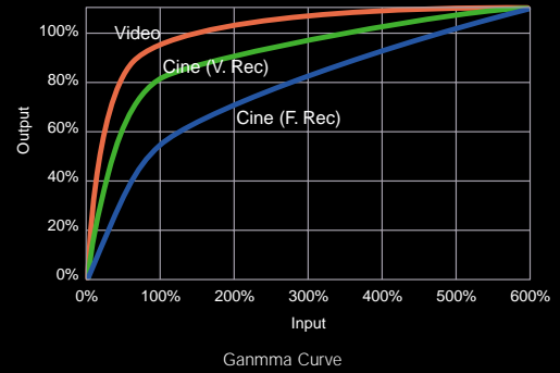
Gamma Curve
